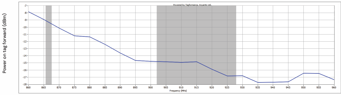
Sensitivity Results from Free Space (dBm)
